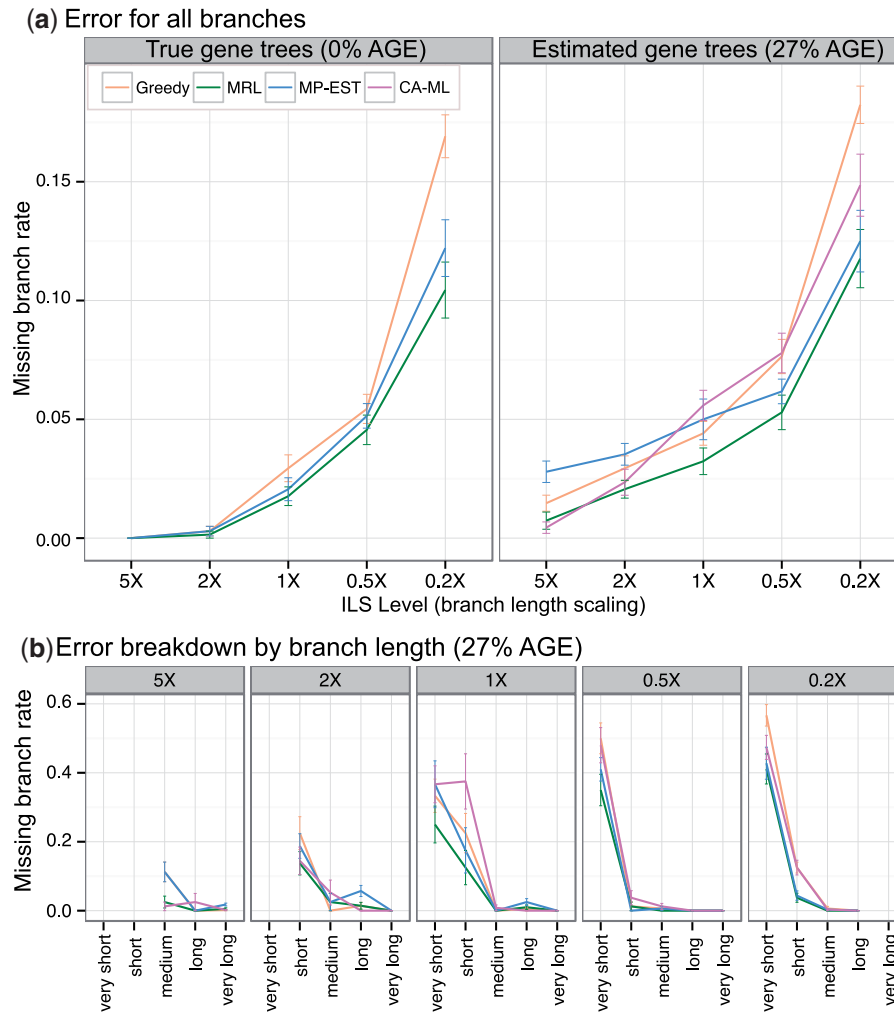
FIGURE 4. Impact of ILS level on species tree estimation. We compare the performance of MRL with Greedy, MP-EST, and CA-ML on the simulated mammalian data set using true and estimated (BestML) gene trees with 26–27% estimation error. Missing branch rate is computed with respect to (a) all branches of the model species tree or (b) various categories of branch length. We show the average tree error (bars indicate standard error) over 20 replicates of 200 genes (see Supplementary Table S1 available on Dryad; http://dx.doi.org/10.5061/dryad.310q3 for SD).
